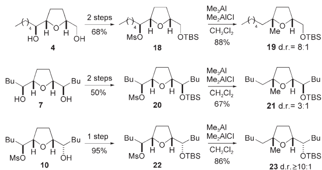
Scheme 6. Stereoselective organometallic addition. OTBS = OSi- t BuMe 2 .
